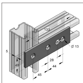
Conector plano 3-taladros 40/5
