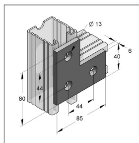
Conector plano forma-L 40/6
