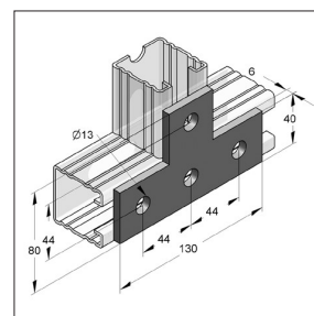
Conector plano forma-T 40/6
