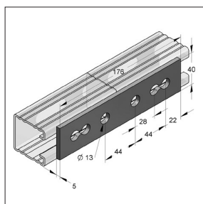
Conector plano 4-taladros 40/5
